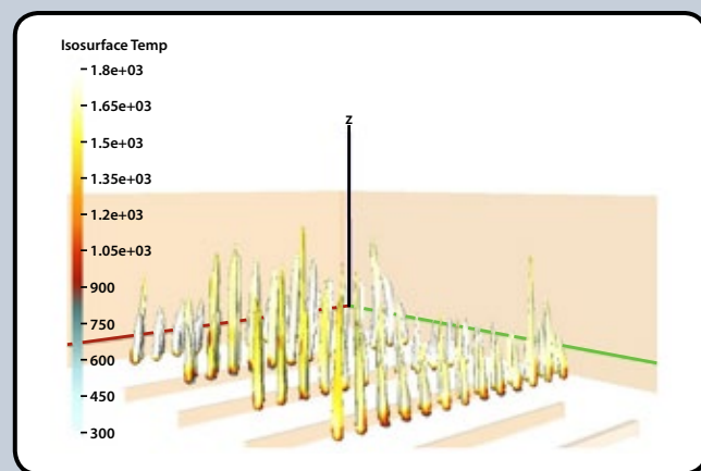
ZEECO CFD Model
